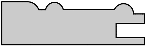
M300 Modified | 2½" wide
