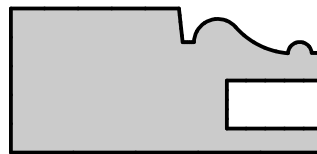
M1901 | 1⅝" wide
