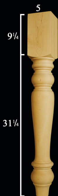
1509 Extended Massive Wilmington 40 1/2 x 5
