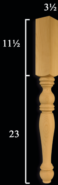
Lynden Island Leg
