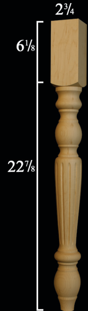
1115 Narrow Modified English Country 29 x 2 3/4
