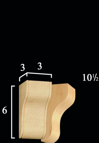
Little Rock Contemporary Corbel 6 x 3 x 3
