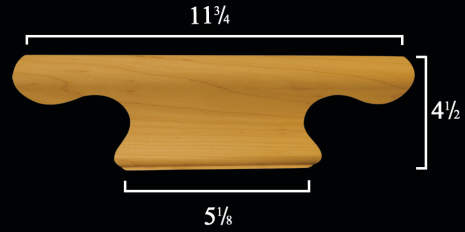
4303 Center Colonial Ogee Foot
