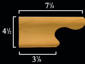
4301 Left Colonial Ogee Foot
