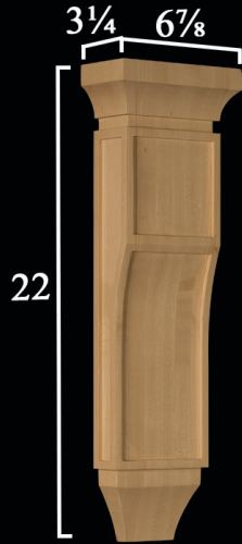
8066 Narrow Mission Bar Corbel 22 x 6 7/8 x 3 1/4
