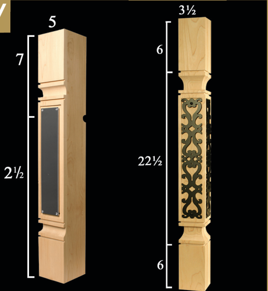
LED Mood Lit Massive Square Mission Island Leg
