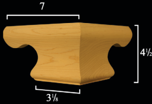
4300 Corner Colonial Ogee Foot
