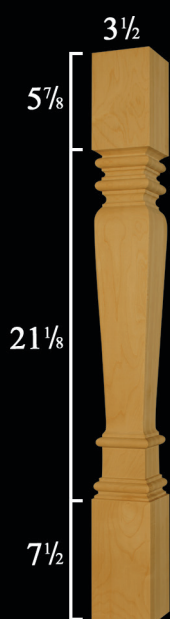
Square Islander Island Post
