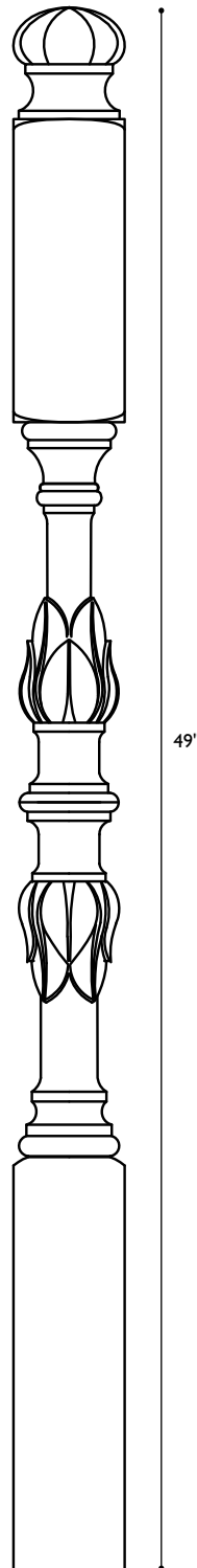
NWL-ALB-3 Newel Hearst Alabaster Large 49" h Top: 3 1/2" sq. Bot: 3 1/2" sq.
